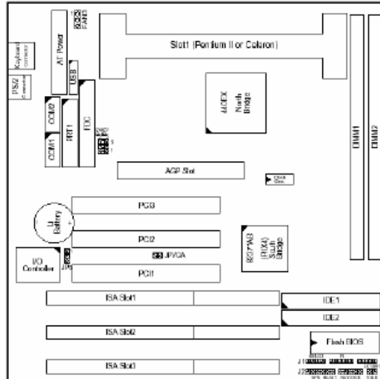
Figure 1-1. Motherboard Layout
